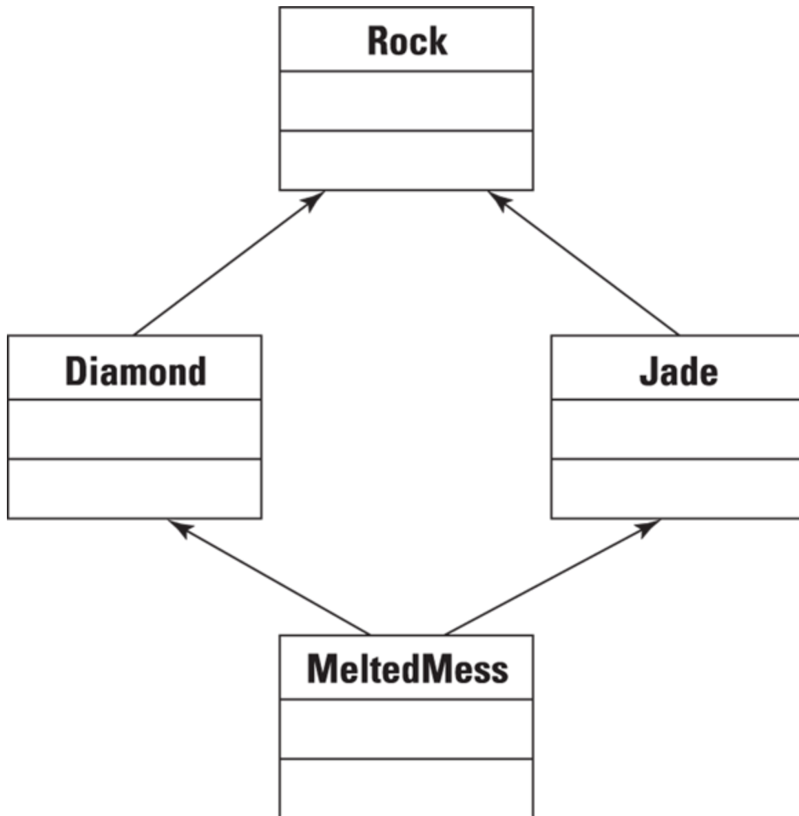
FIGURE 4-1: Using diamond inheritance can be hard.
