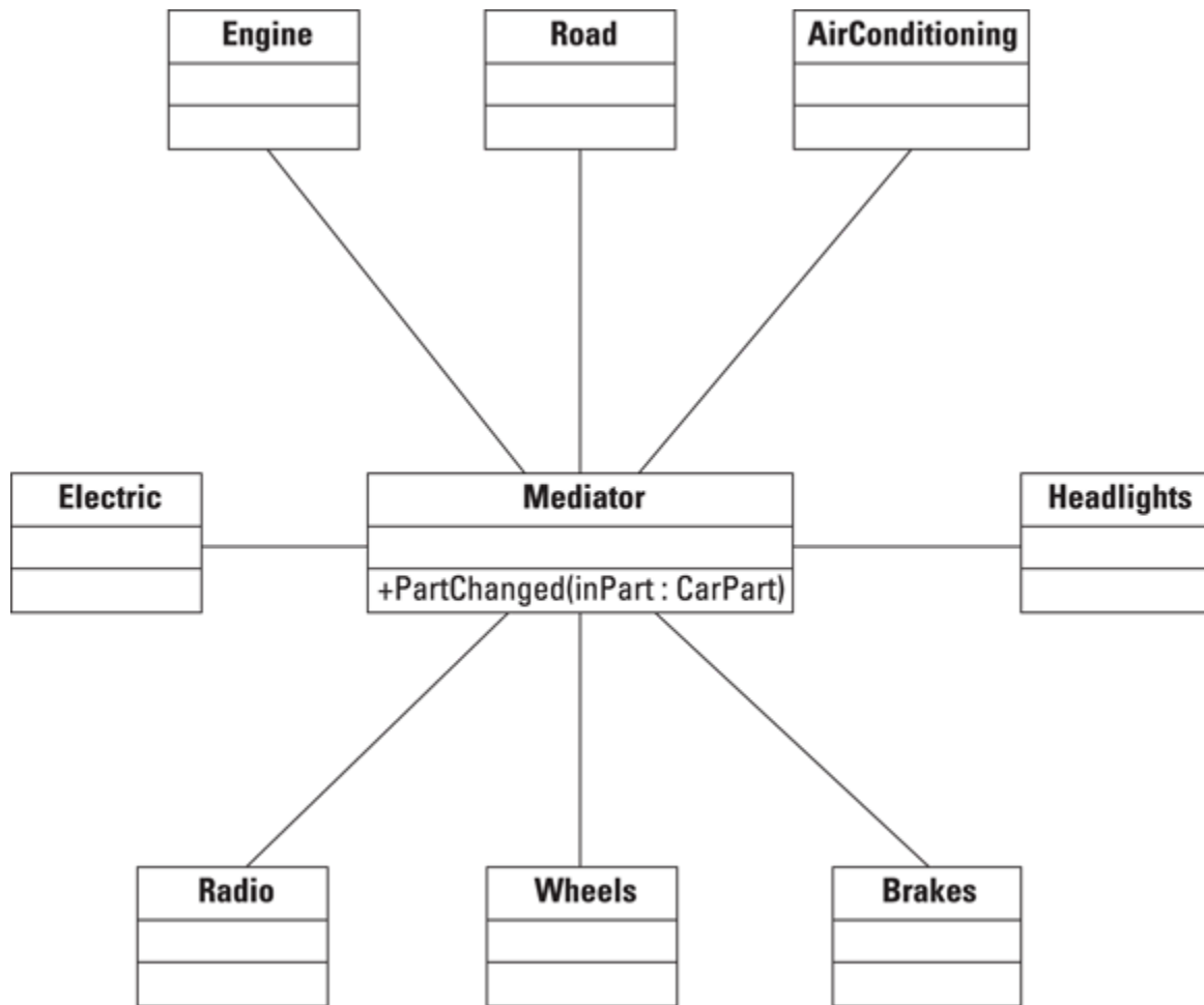
FIGURE 4-2: A mediator certainly cleans things up!
