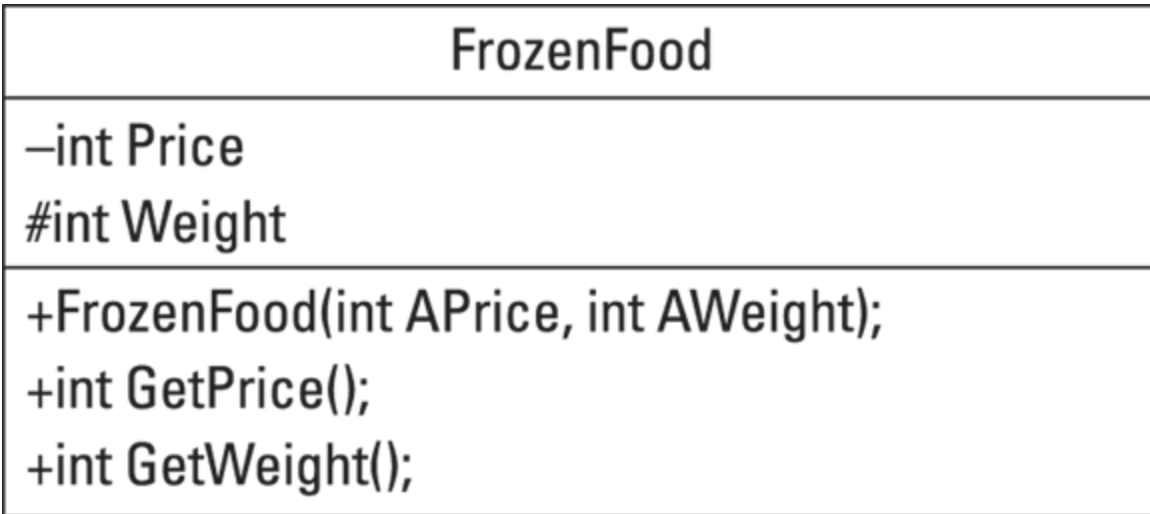
FIGURE 3-3: You can draw a class by using a box divided into three horizontal sections.
